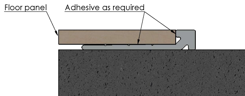
Typical installation detail
