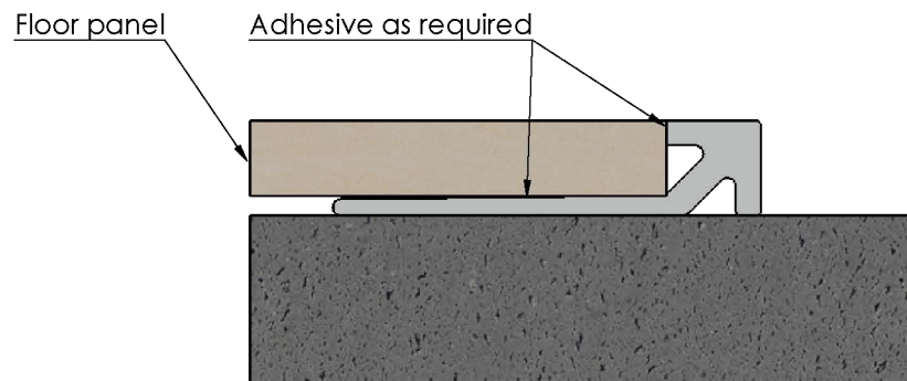
Typical installation detail
