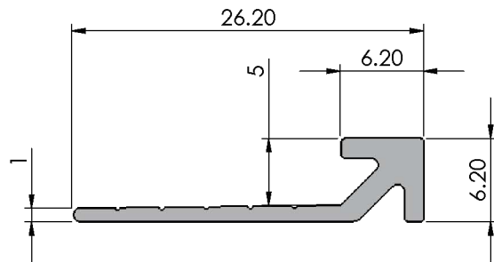
Section view
