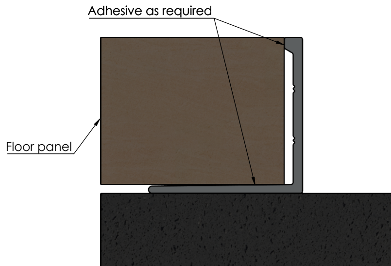
Typical installation detail
